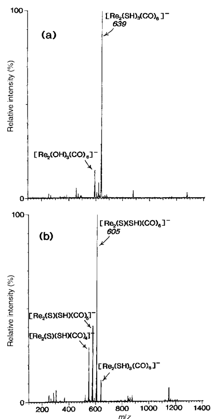
Fig. 2 Negative ion ES spectra of [\text{Re}_2(\mu\text{-SH})_3(\text{CO})_6]^- (generated from [\text{Re}_2(\mu\text{-OH})_3(\text{CO})_6]^- 1 and H 2 S) in MeCN solution at cone voltages of (a) 5 and (b) 50 V, showing fragmentation by loss of H 2 S and CO.
