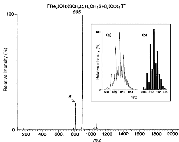
Fig. 3 Negative ion ES spectrum (cone voltage 5 V) of [Re 2 (μ-OH) 2 (CO) 6 ] - 1 and benzene-1,4-dimethanethiol, HSCH 2 C 6 H 4 CH 2 SH, after 1 week reaction in MeCN. The inset shows a comparison of (a) experimental and (b) calculated isotope distribution patterns for the aggregate dianion 8 at m/z 811.
